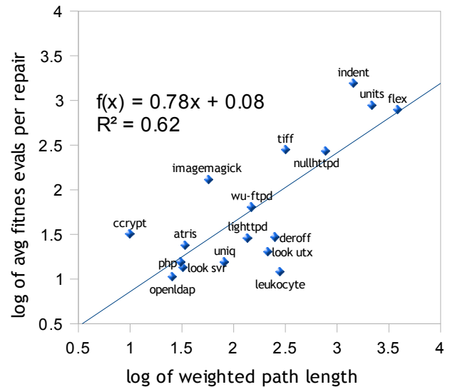
Figure 1: GP search time scales with weighted path size. Data are shown for 18 programs successfully repaired by GP ( gcd and zune examples omitted), with best linear fit. The x-axis is the base-10 logarithm of the weighted path length, and the y-axis shows the logarithm of the total number of fitness evaluations performed before the primary repair is found (averaged over 100 runs).
