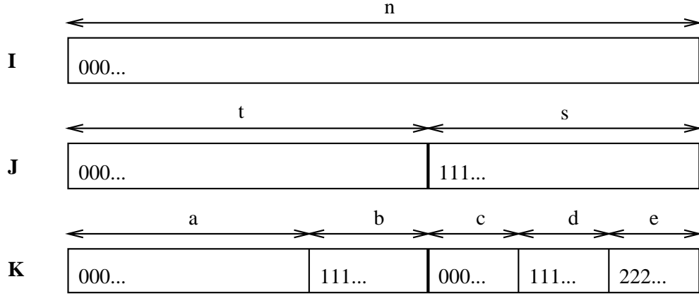
Figure 5: This figure shows the five groupings of the symbols of K , and how these groups relate to the groupings in I and J .
