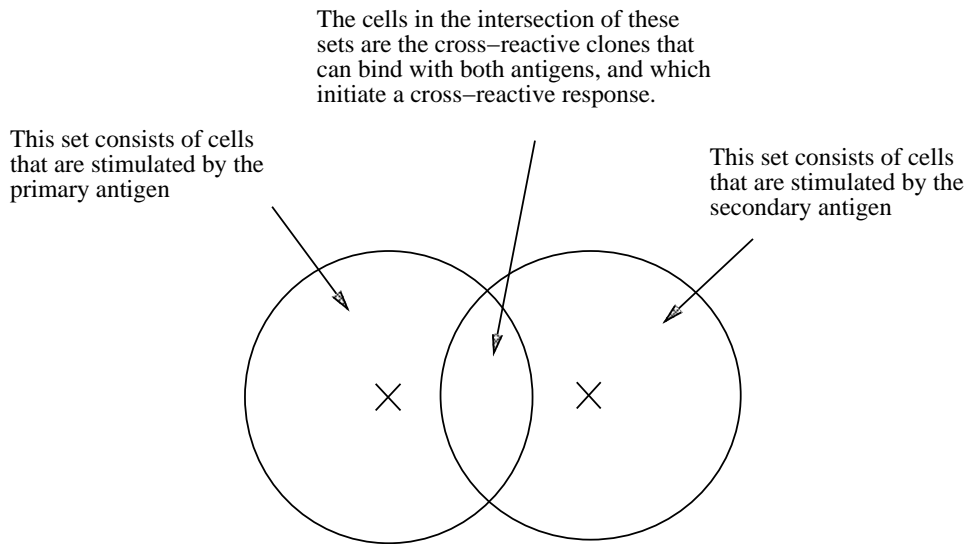
Figure 1: The cells that cause a cross-reactive response are those in the intersection of the set of cells stimulated by the primary antigen and the set of cells stimulated by the secondary antigen.
