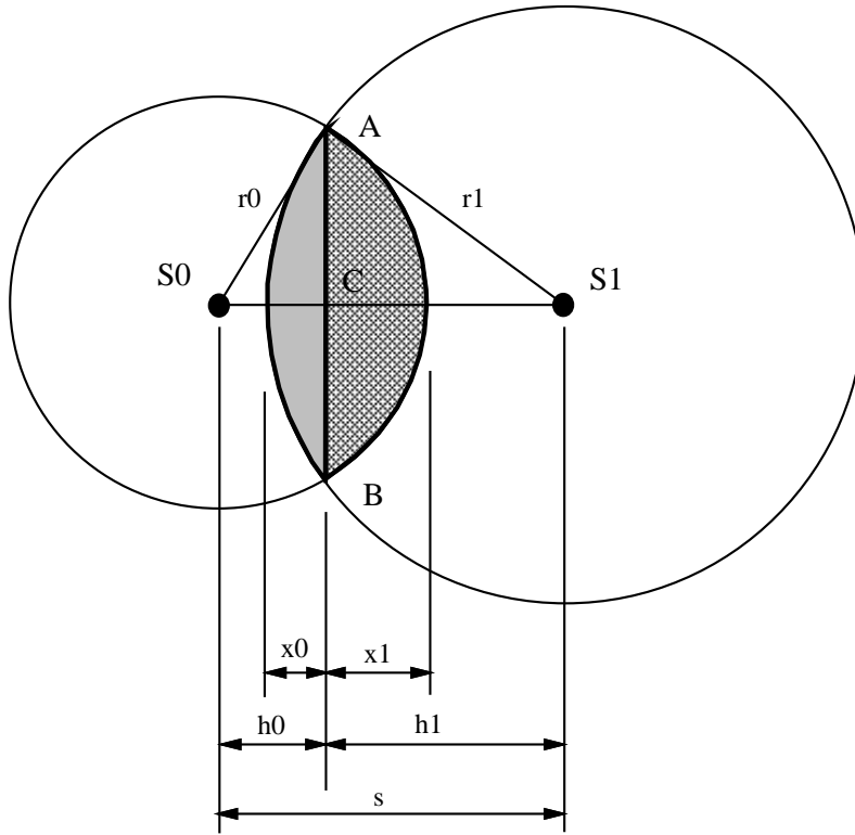
Figure 6: The two shaded segments in this figure, when added together, form the intersection of the balls. The volume of a segment is calculated by integrating along the line S_0S_1 . The key to the calculation is that the integrand is a ball in the next lower dimension whose radius is the distance from S_0S_1 to the circumference of the segment's circle (which varies as x moves along S_0S_1 during the integration).
