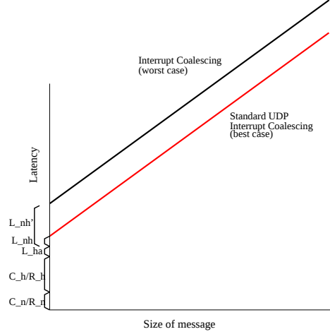
Figure 3. Extensible Message-Oriented Of-flood - Latency
