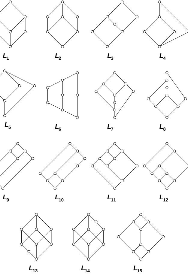
Figure 1: All Covers of the Least Non-Modular Lattice N_5
