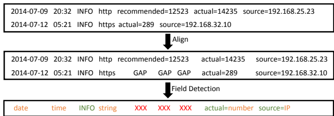
Figure 4: An example of how Algorithm 2 works.
