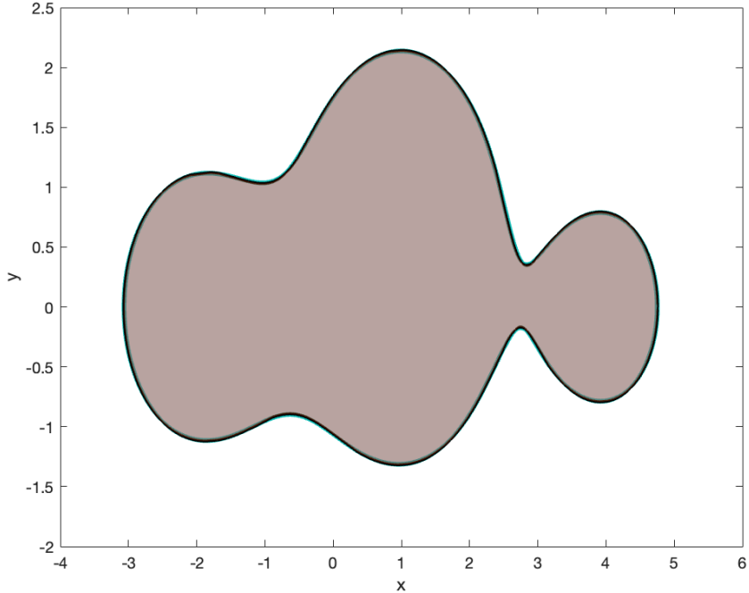
Fig. 7. BOUNDARY-SKETCH for \lambda = 0.000001 , the green border marks the shape boundary sandwiched by the inner and outer robots.
