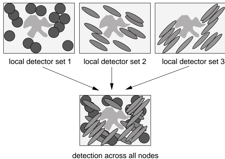
Figure 6: Representation changes are equivalent to “shape” changes for detectors. The problem of holes can be ameliorated by using a different representation for each detection node. There are different holes for different representations, or equivalently different shaped detectors can cover different parts of the nonself space, for a global reduction in holes.
