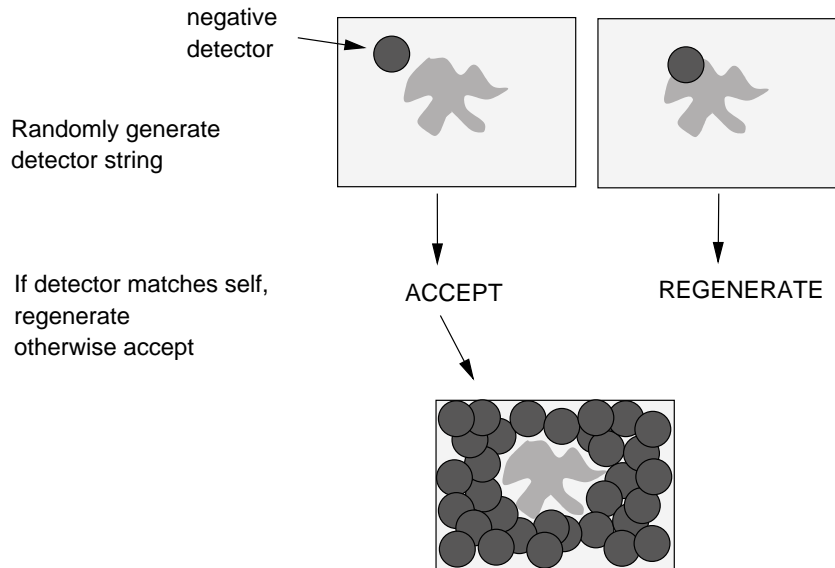
Figure 3: The negative selection algorithm. Candidate negative detectors (represented by dark circles) are generated randomly, and if they match any string in the self set (i.e., if any of the points covered by the detector are in the self set), they are eliminated and regenerated. This process is repeated until we have a set of valid negative detectors that do not match any self strings.
