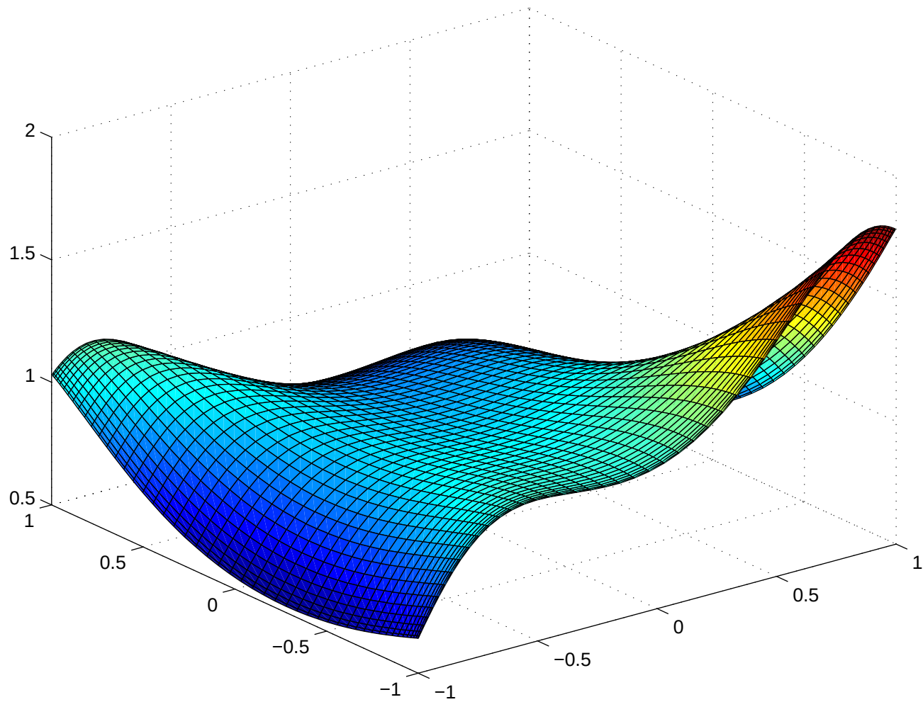
Jacobian
