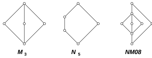
Figure 2: Lattices M_3 , N_5 , NM_8
