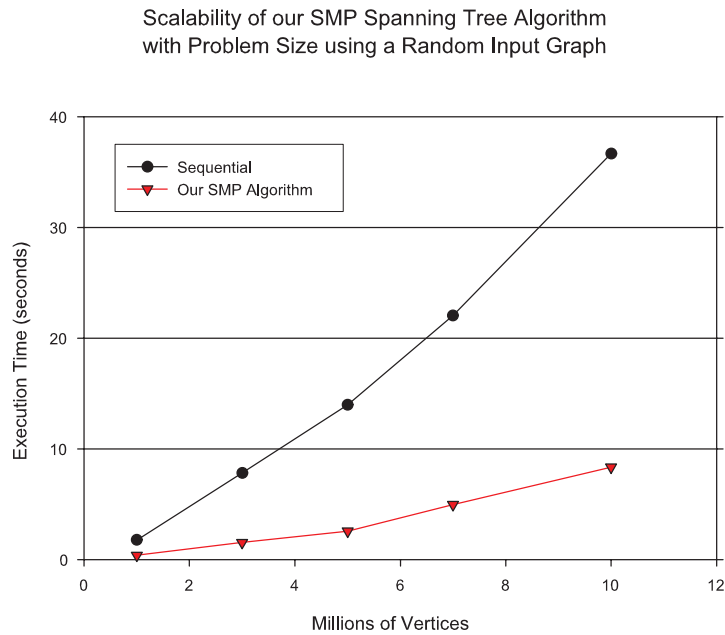
Figure 6: This plot shows the scalability of our SMP spanning tree algorithm using p = 8 processors compared with the sequential algorithm for a random graph. For these experiments, the speedup of the parallel algorithm compared with the sequential approach is between 4.5 and 5.5.
